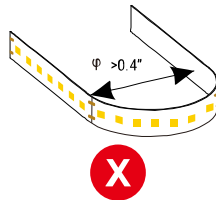
Do not bend less than the minimum bending diameter
